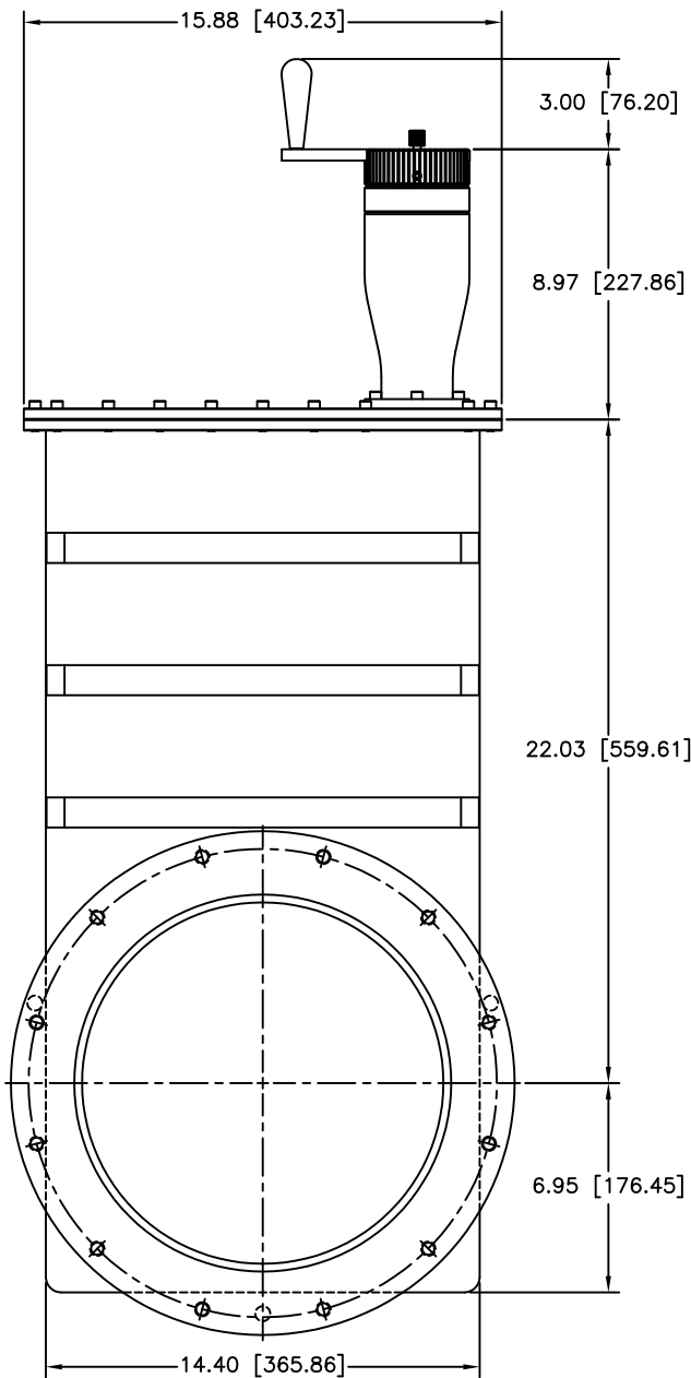
CARRIAGE SIDE
