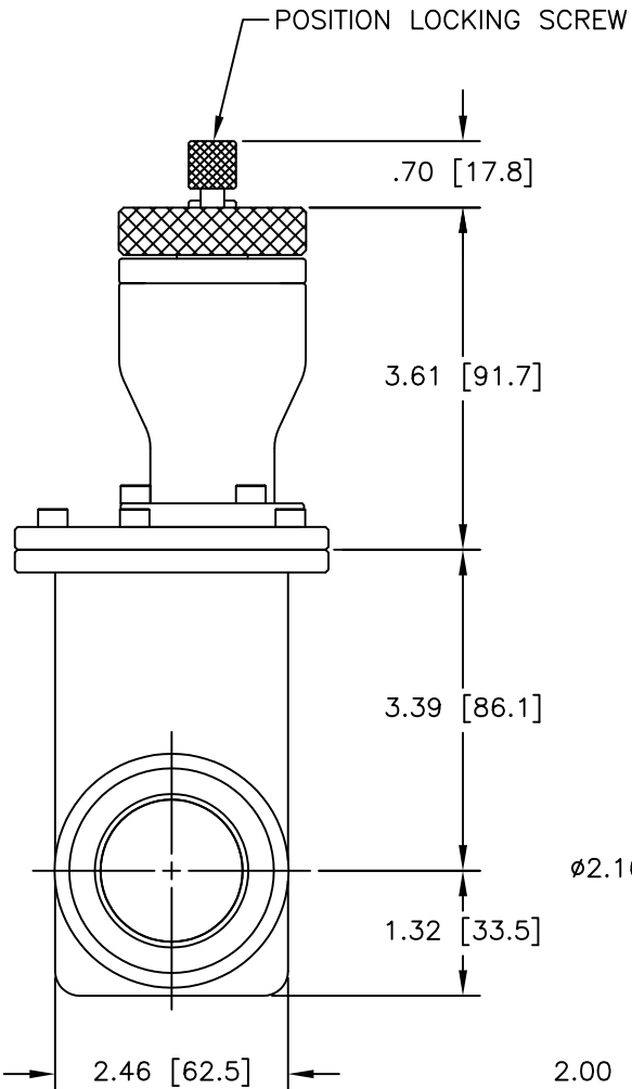
CARRIAGE SIDE
